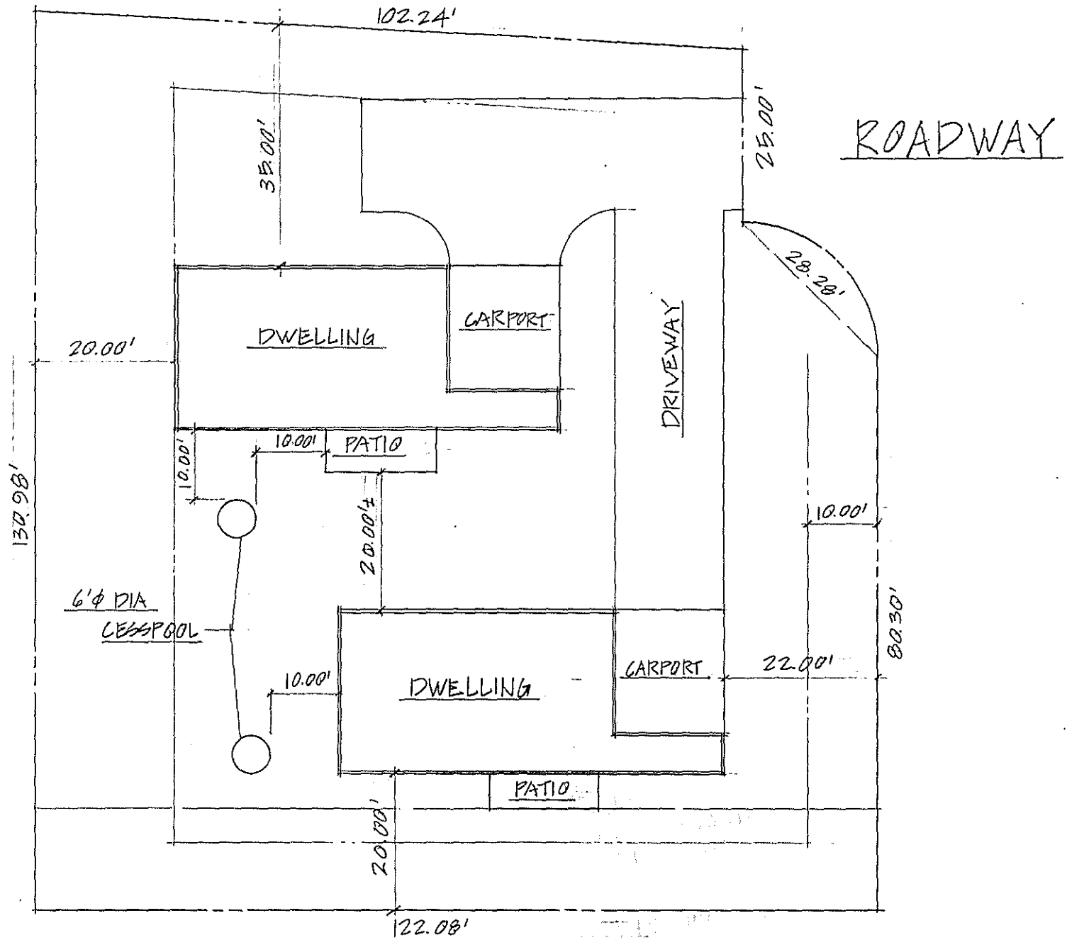
PLOT PLAN 5/6" = 20.00'
