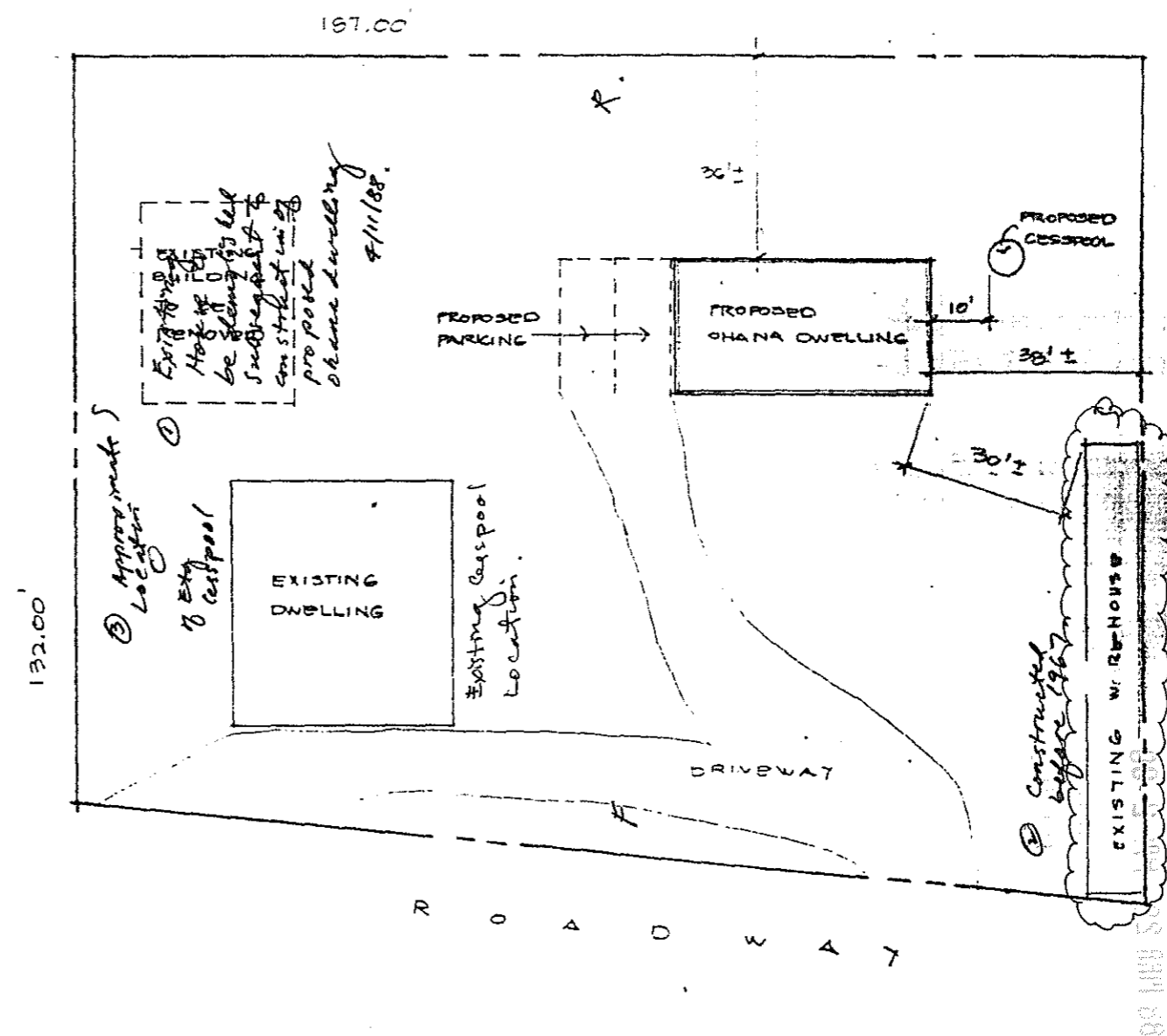
PLOT PLAN SCALE: 1" = 30.00'
