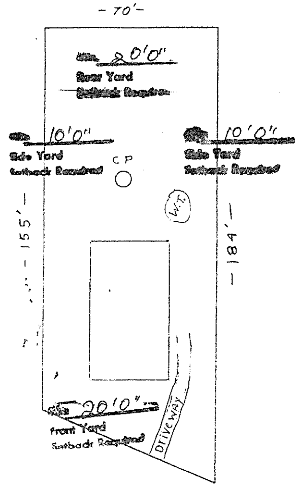
PLOT PLAN SCALE = 1/4" = 10 ft.
