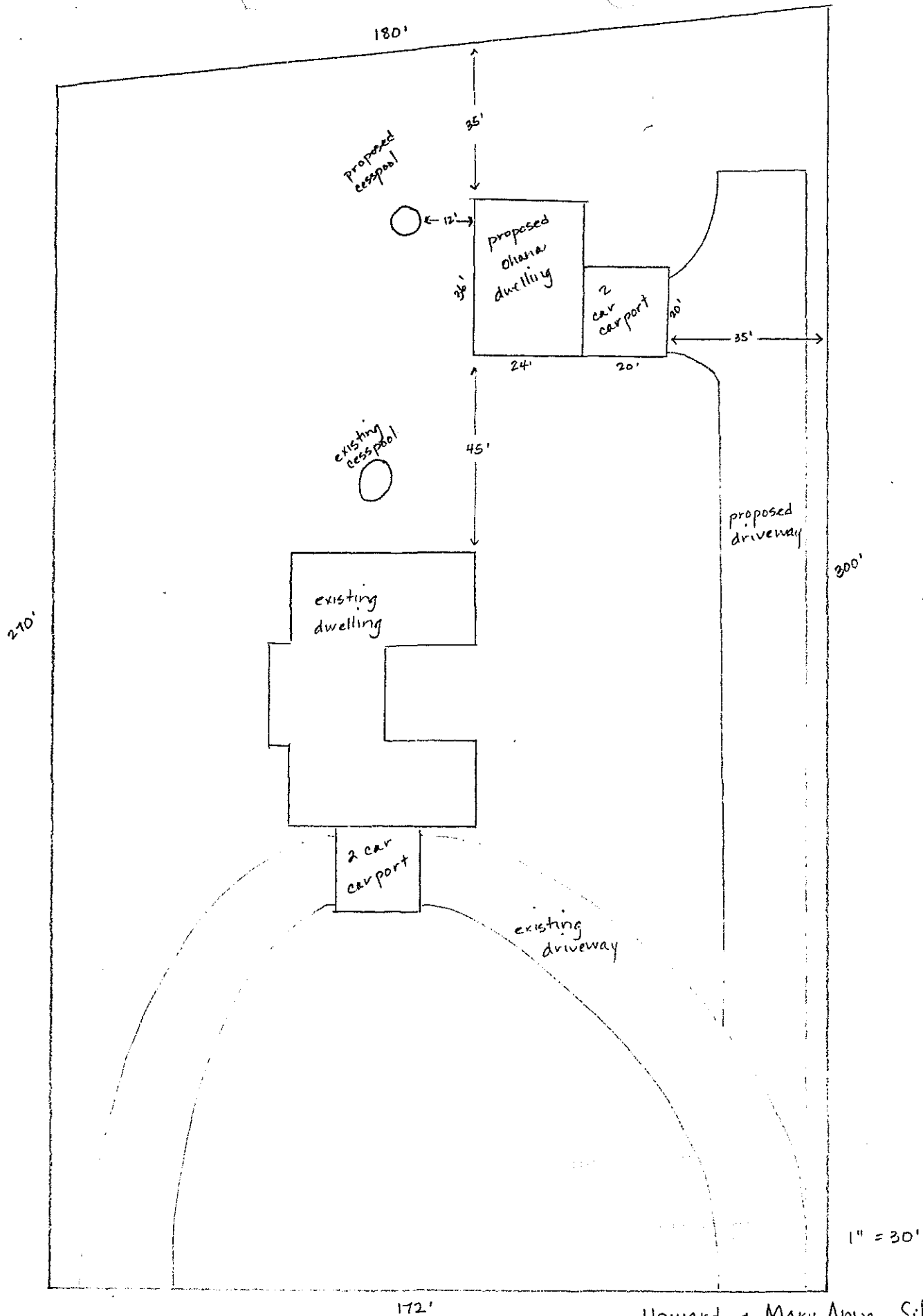
Ohara Dwelling Plot Plan
