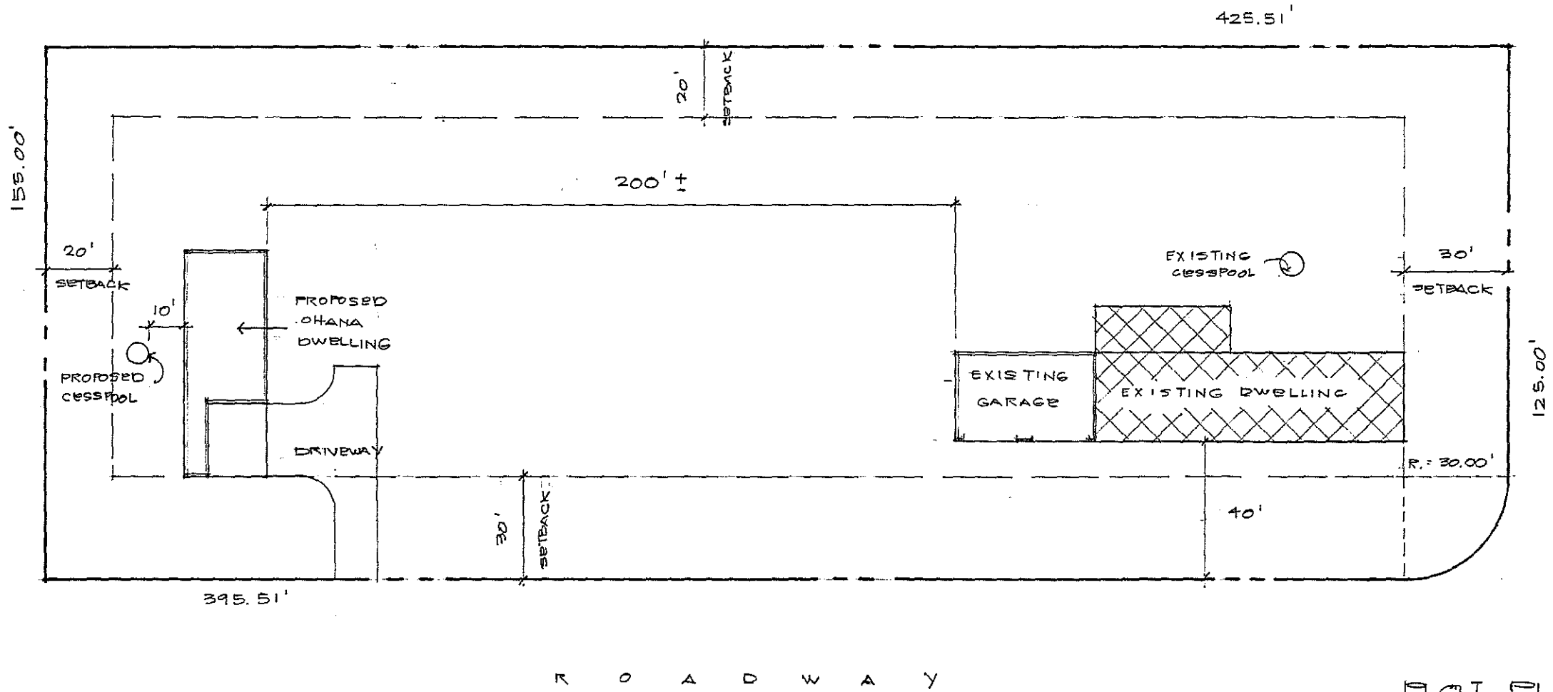
PLOT PLAN SC.: 1" = 40.00'
