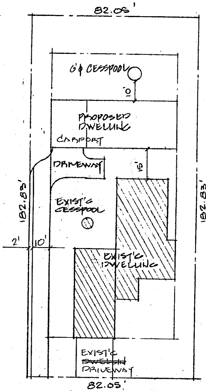
PLOT PLAN 1" = 30'0"
