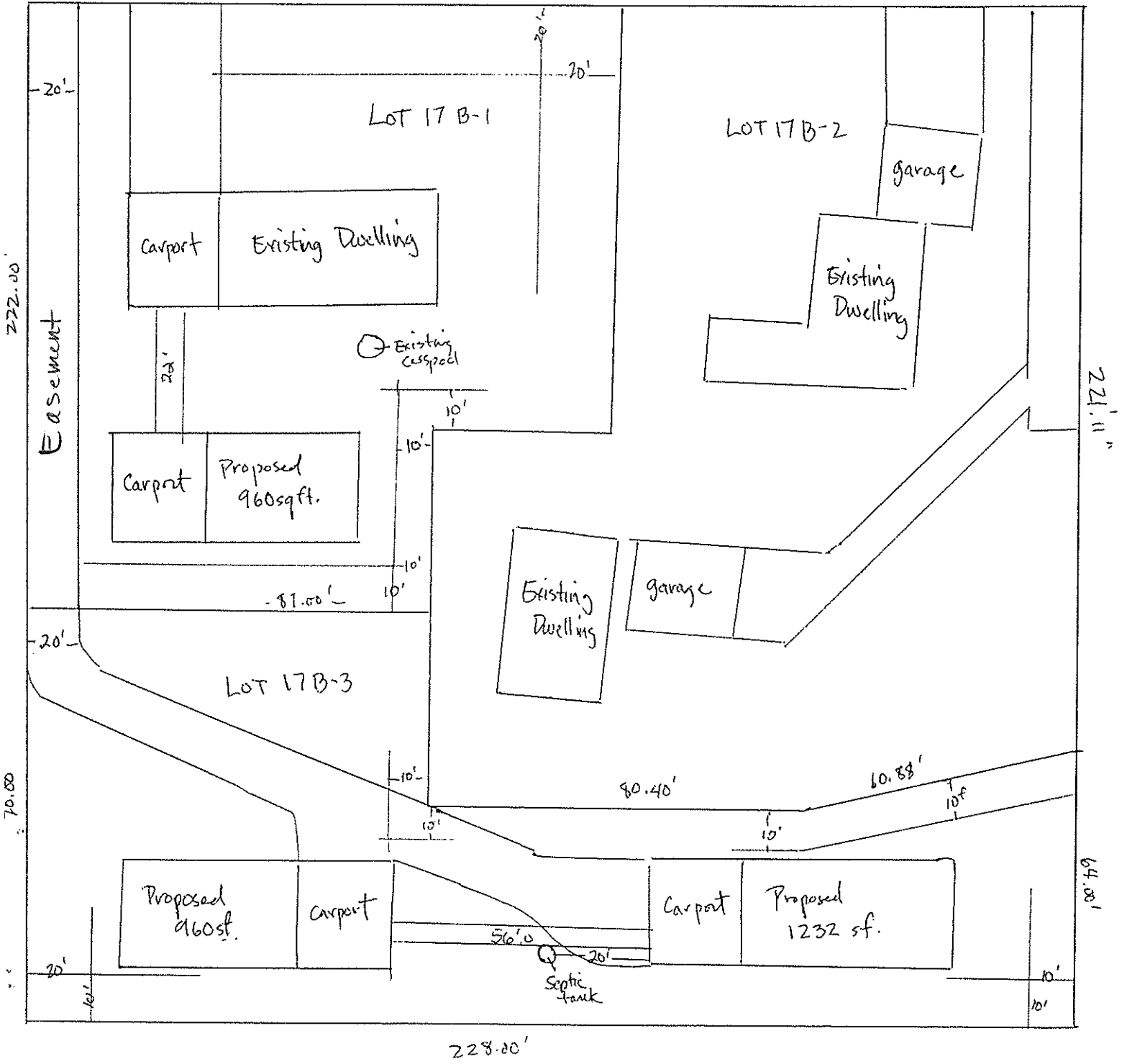
PLOT PLAN : Scale 1" = 30.0" TMK: 2-4-14:62 Lots 17-B1, 17-B2, 17-B3
