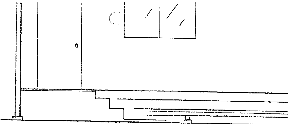
LEFT ELEVATION SC. 1/4" = 1'
