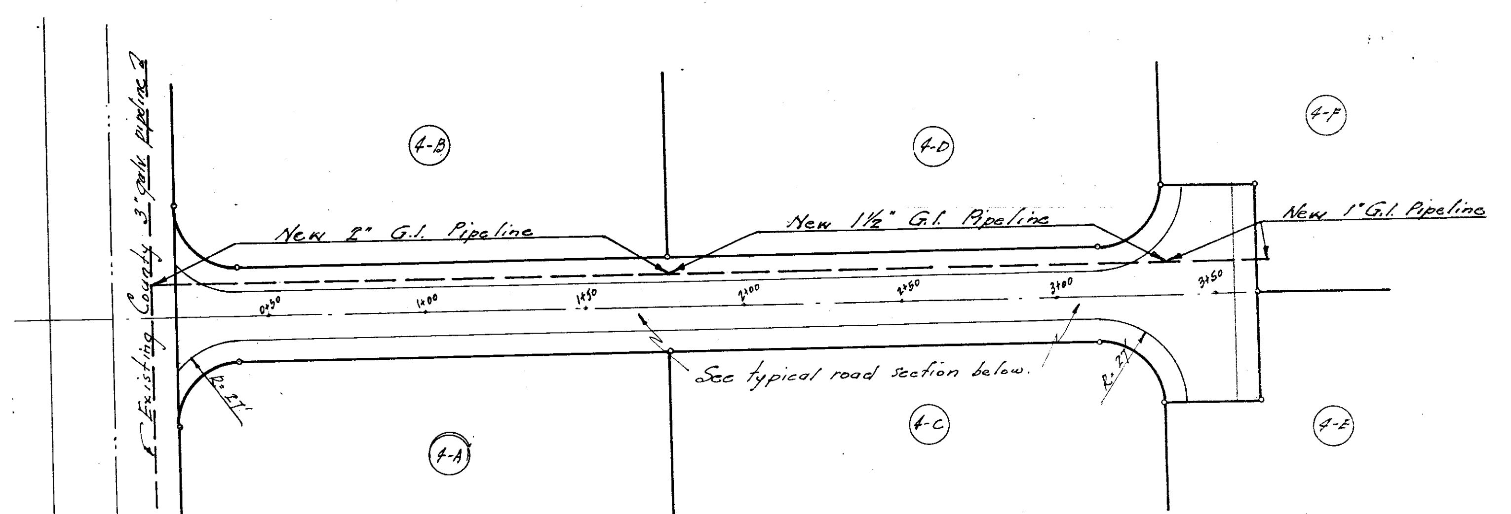
PLAN SHOWING ROAD AND WATER LAYOUT SCALE 1" = 30'-0"
