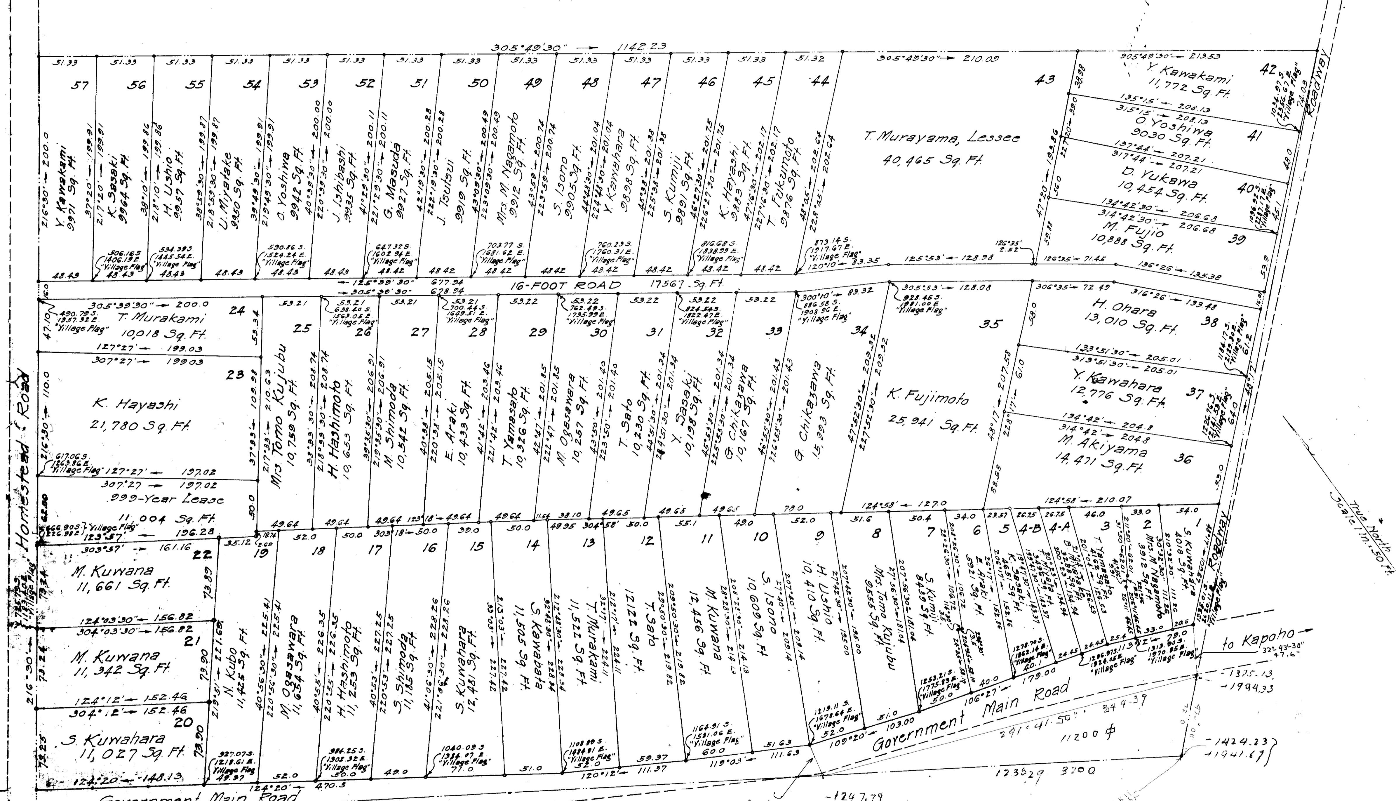
Plan Showing SUBDIVISION OF GRANT 4729 TO P. CARY Nanawale Homesteads Puna - Hawaii Scale 1 in. = 50 Ft.
